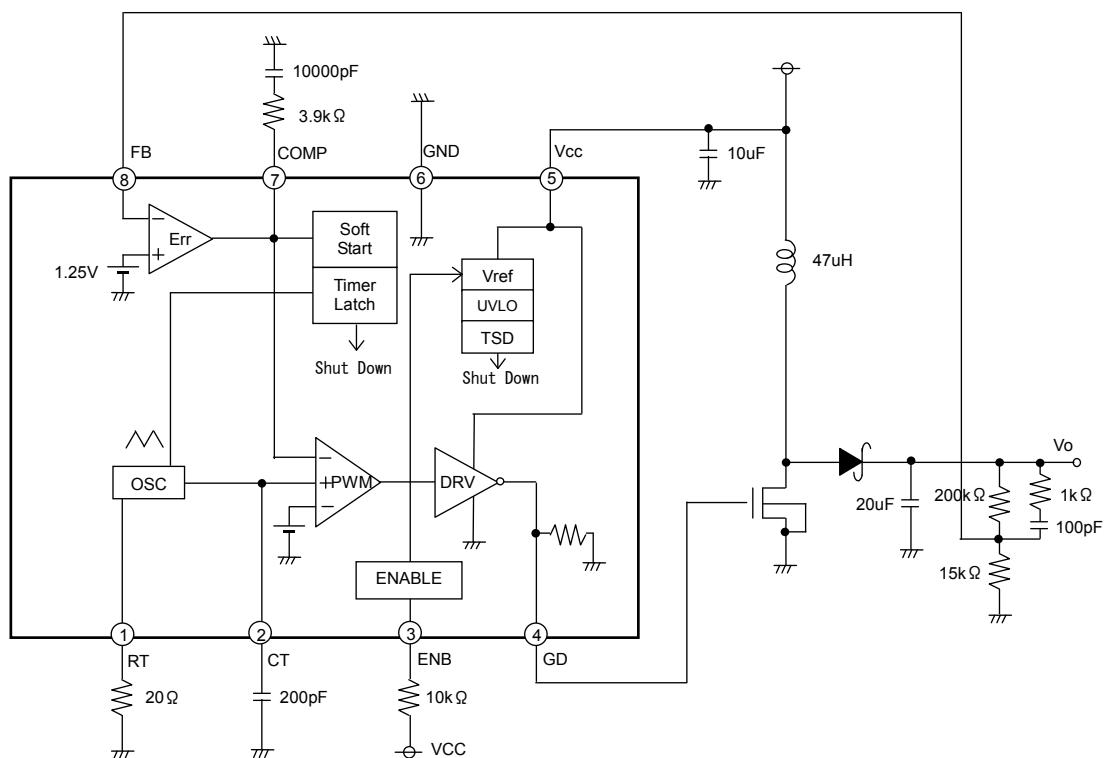
Fig.21 Block Diagram / Application Circuit (BD9306AFVM)
