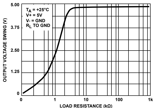
FIGURE 8. OUTPUT VOLTAGE SWING vs LOAD RESISTANCE
