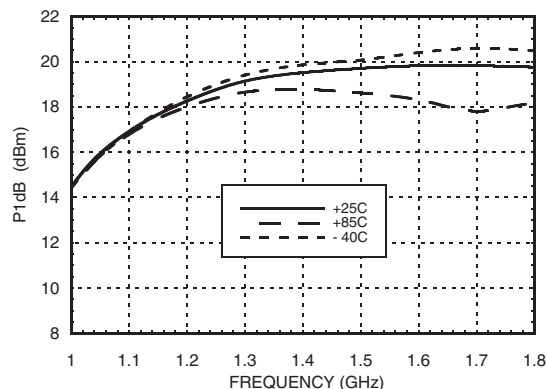
Output P1dB vs. Temperature [1]
