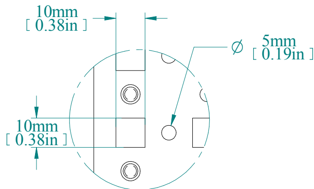
DETAIL A
