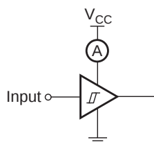
Figure 2. I CCD Test Circuit
