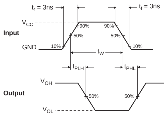
Figure 3. AC Waveforms
