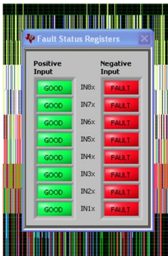
Figure 20. Fault Status Indicator
