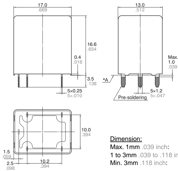
External dimensions
