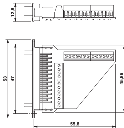
D-SUB contact insert
