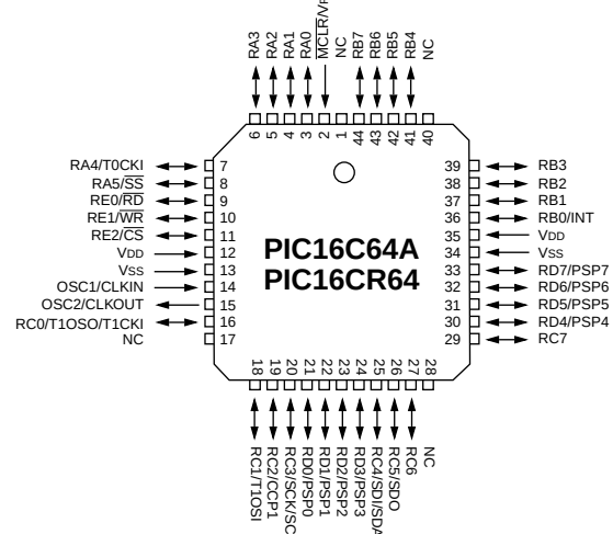
PLCC
