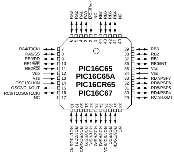
PLCC
