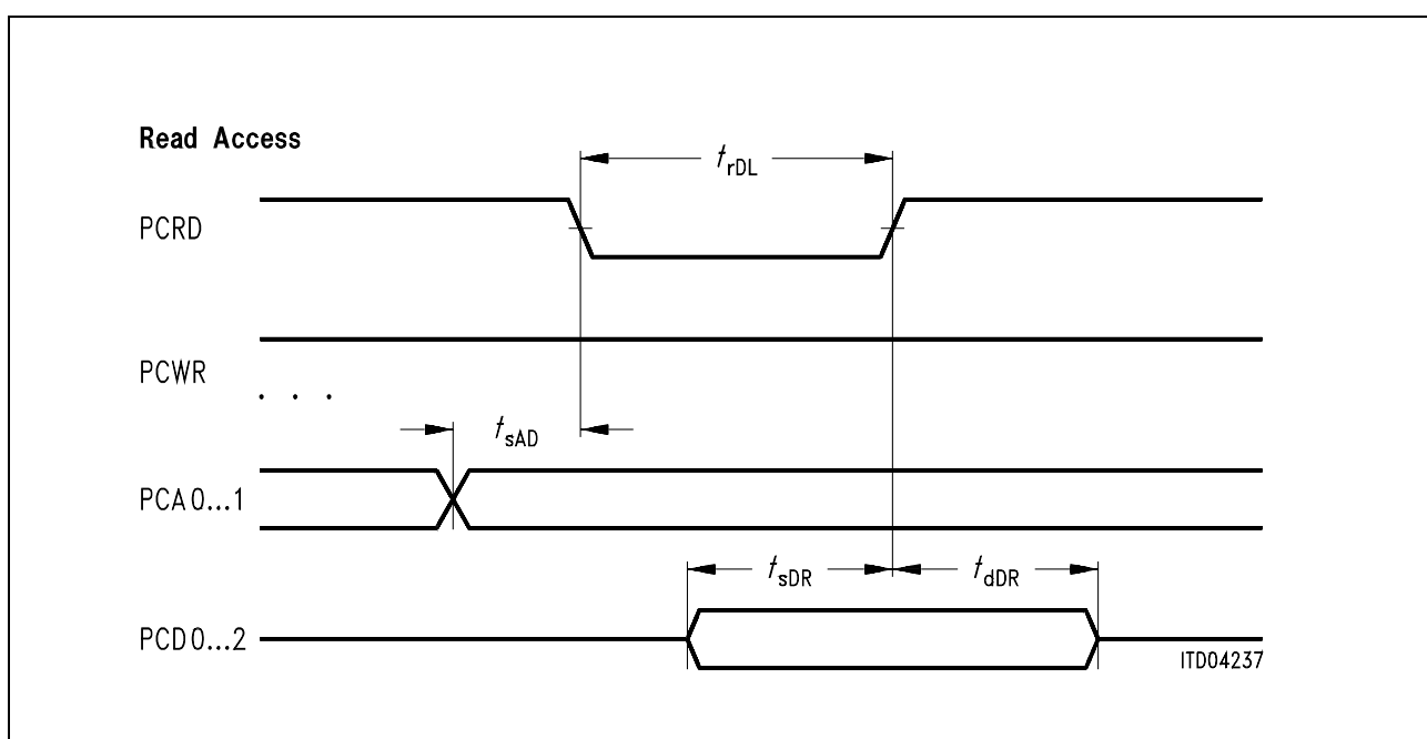
Figure 62 Dynamic Characteristics of Power Controller Read Access
