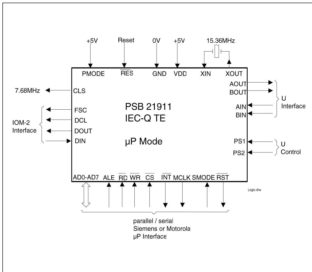
Figure 2 Logic Symbol \mu P Mode
