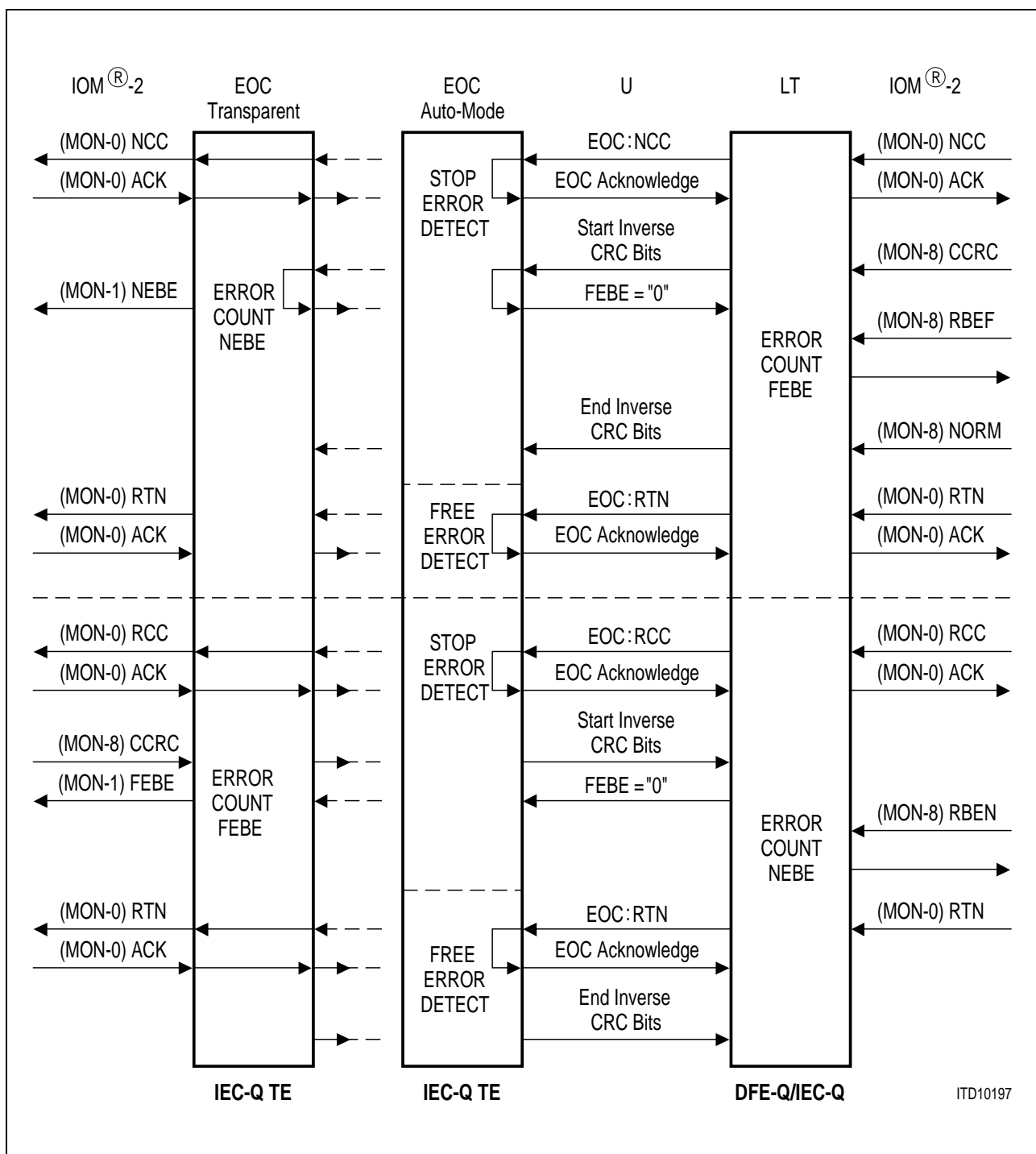
Figure 18 Block Error Counter Test
