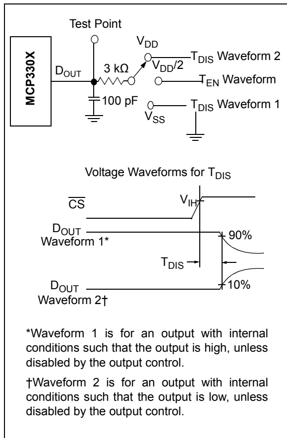
FIGURE 1-3: Load circuit for T_{DIS} and T_{EN} .
