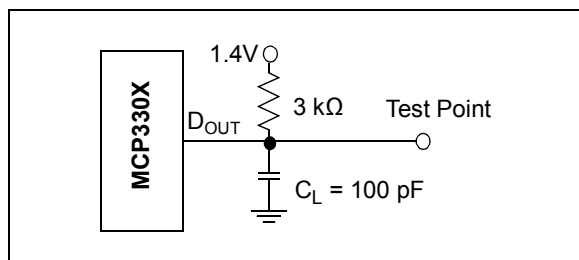
FIGURE 1-2: Load Circuit for T_R , T_F , T_{DO} .
