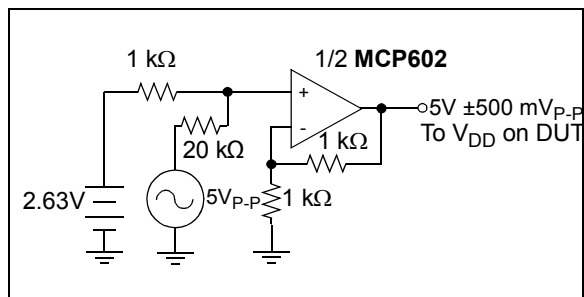
FIGURE 1-4: Power Supply Sensitivity Test Circuit (PSRR).
