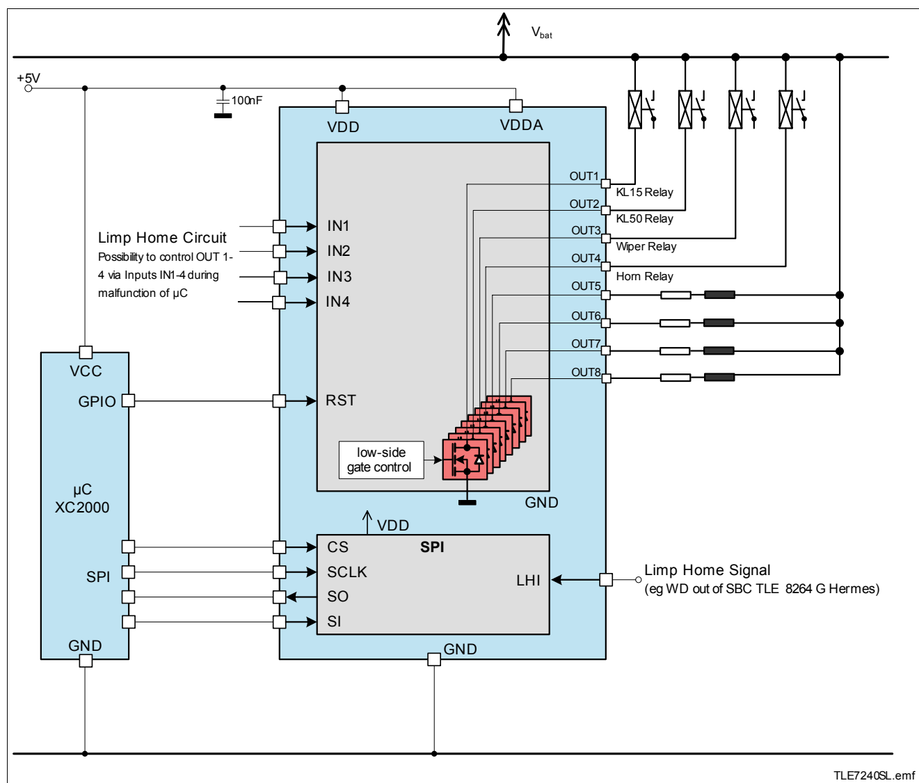
Figure 13 Application Diagram
