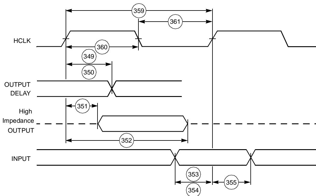
Figure 2-36. PCI Timing
