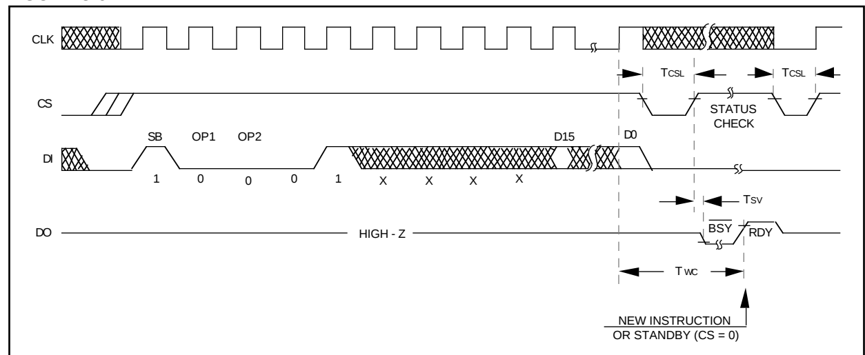
FIGURE 3-6: WRITE ALL
