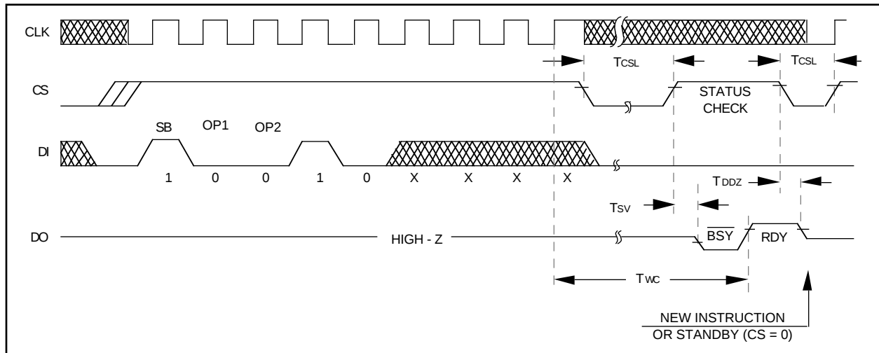
FIGURE 3-5: ERASE ALL
