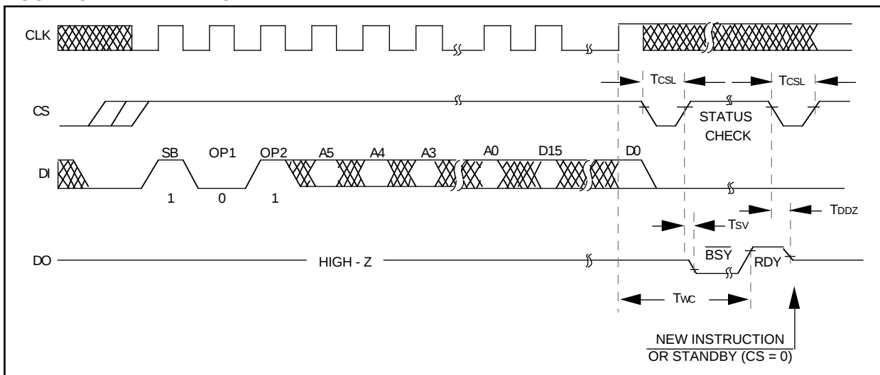
FIGURE 3-2: WRITE MODE
