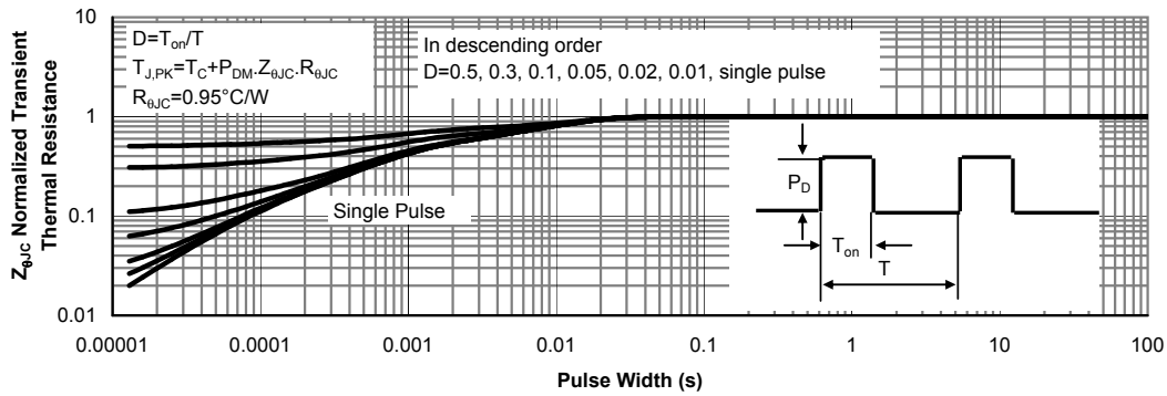
Figure 11: Normalized Maximum Transient Thermal Impedance for AOT5N60 (Note F)
