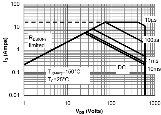
Figure 9: Maximum Forward Biased Safe Operating Area for AOT5N60 (Note F)
