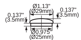
OB-31 Mounting Hole Rubber Plug
