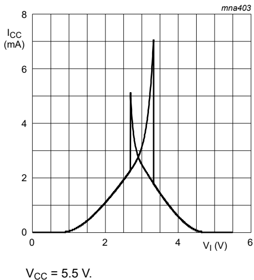
Fig. 8. Typical 74AHC3G14-Q100 transfer characteristics
