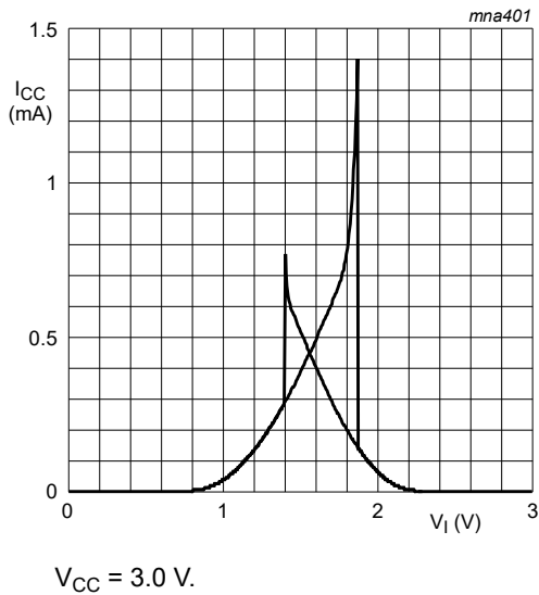
Fig. 6. Typical 74AHC3G14-Q100 transfer characteristics
