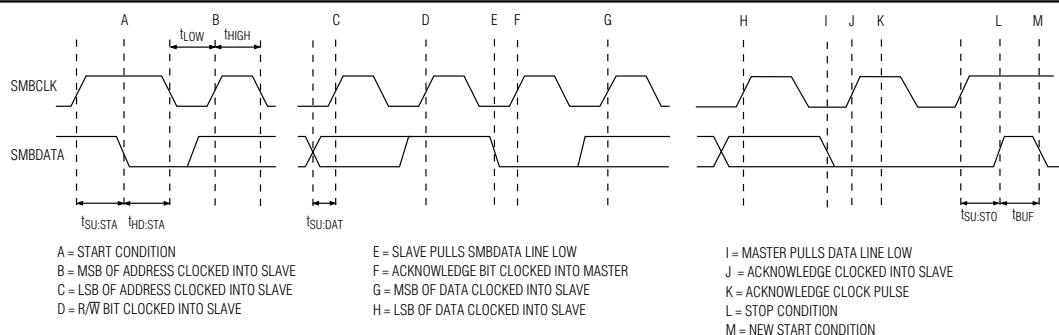
Figure 2. SMBus Write Timing Diagram
