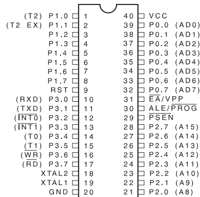
PDIP
