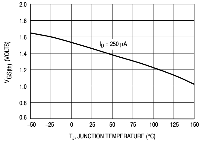
Figure 10. Threshold Voltage
