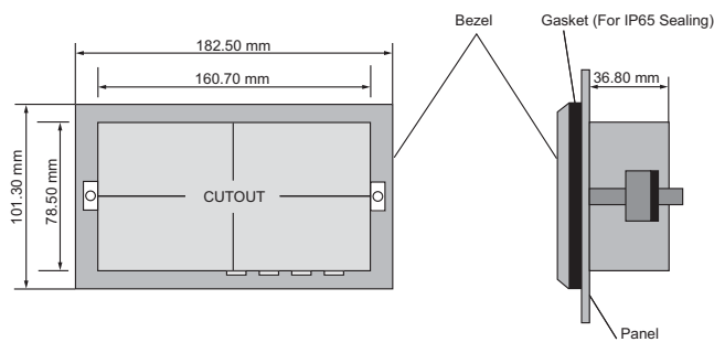
HG1X-452/HG1X-422/HG1X-822 Dimensions/Panel Cutout
