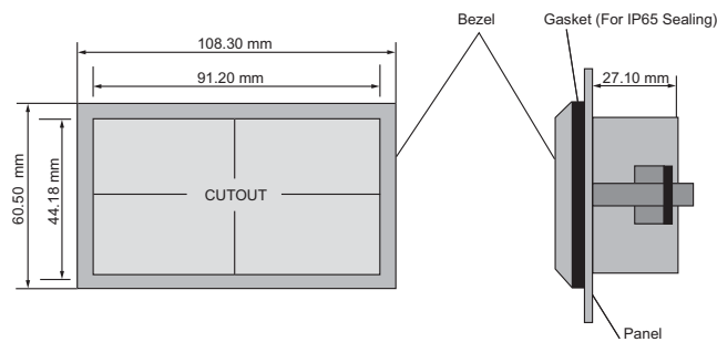
HG1X-252/HG1X-222 Dimensions/Panel Cutout
