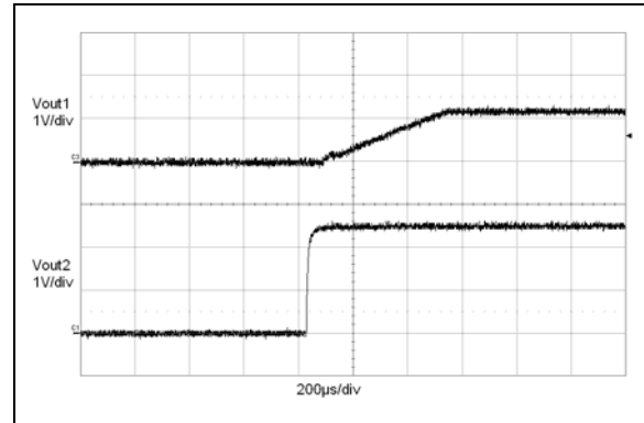
FIGURE 2-42: Start-up Waveforms (TC1304).
