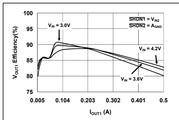
FIGURE 2-8: V_{OUT1} Output Efficiency vs. I_{OUT1} ( V_{OUT1} = 1.8\text{V} ).
