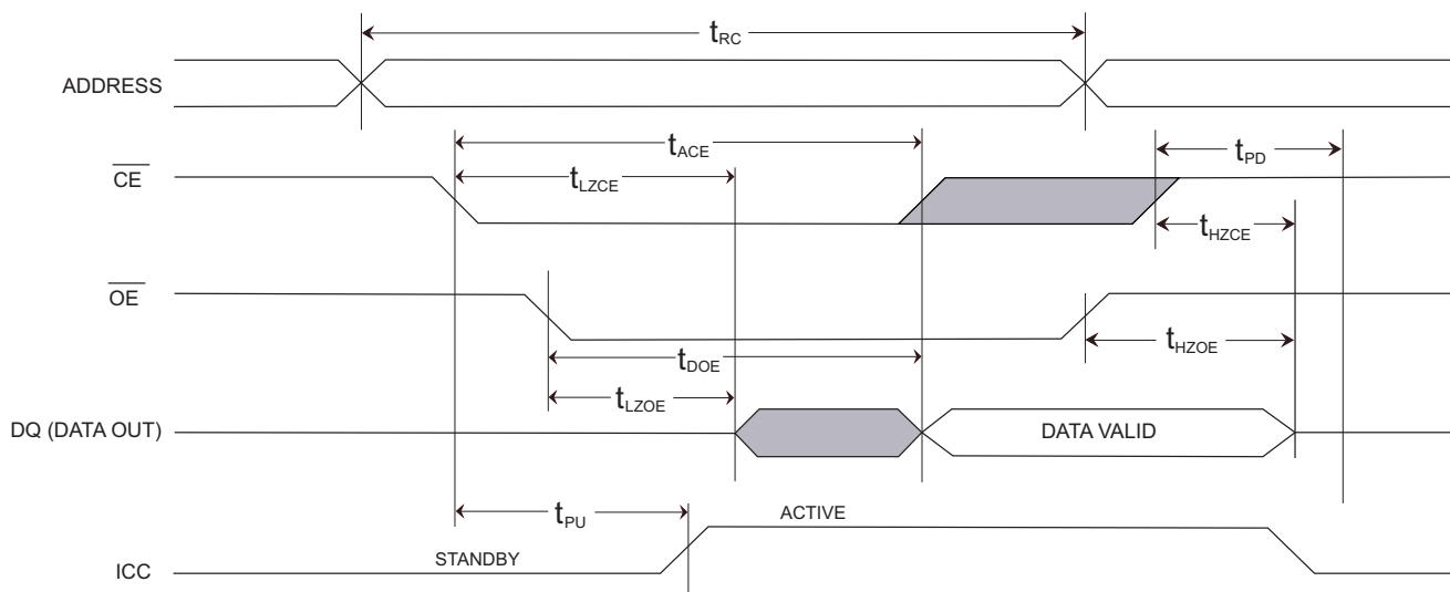
Figure 7. SRAM Read Cycle Number 2: \overline{\text{CE}} Controlled [3,12]
