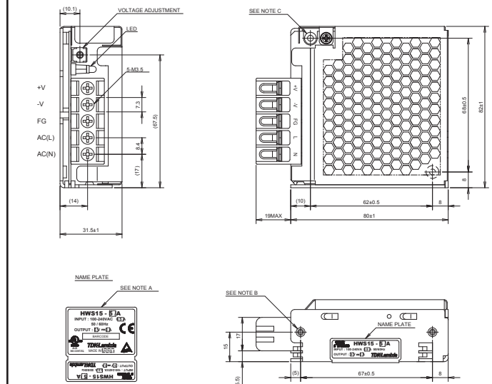
HWS15 Outline Drawing
