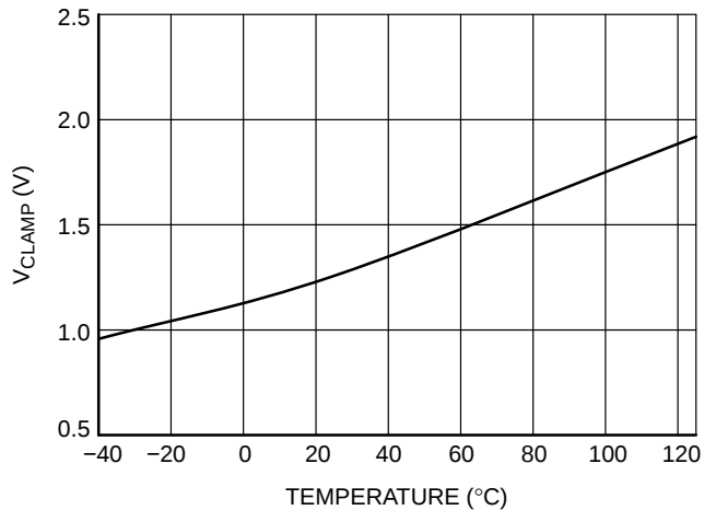
Figure 17. V_{CLAMP} at 0.5 A (NCx5703A Only)
