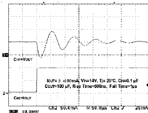
Load Transient
