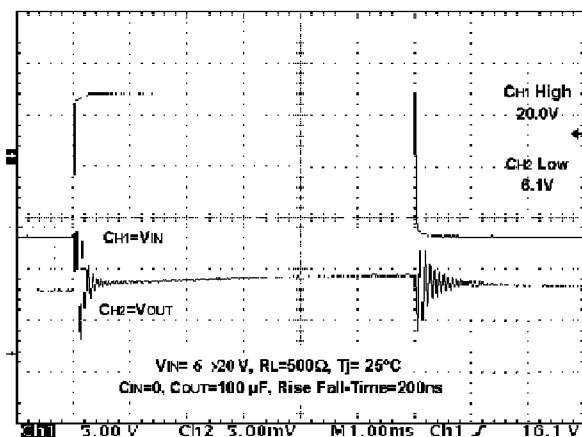
Line Transient
