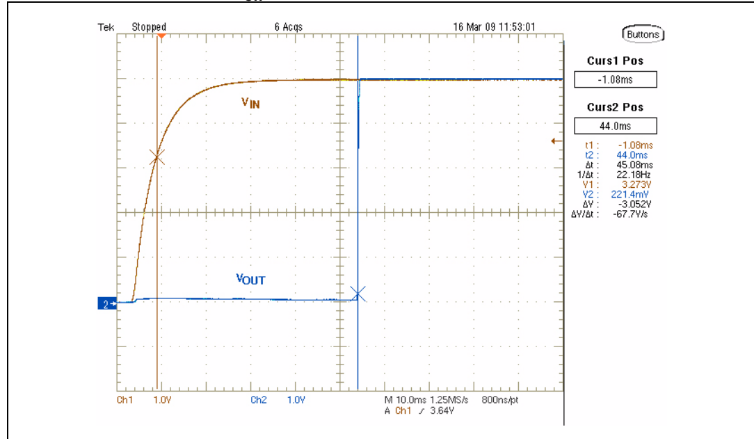
Figure 10. Startup delay, t_{on}
