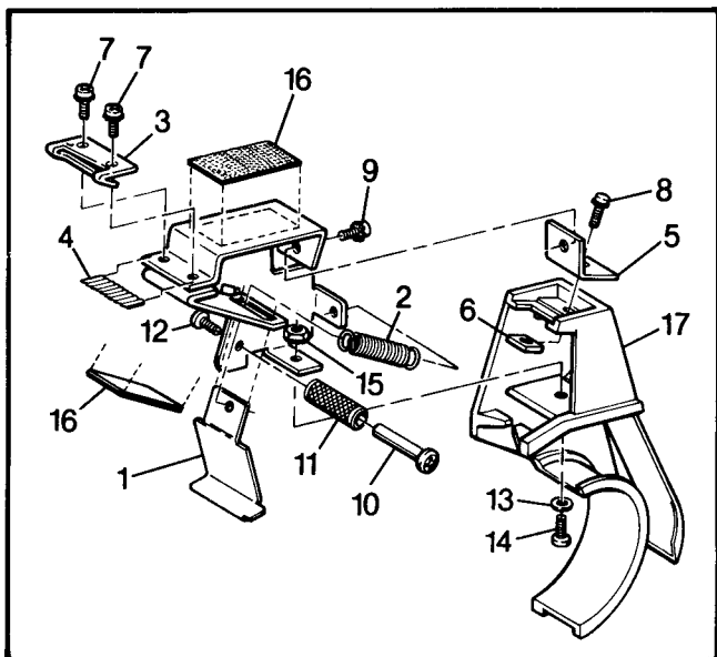
Figure 6 — Replacement Parts.
