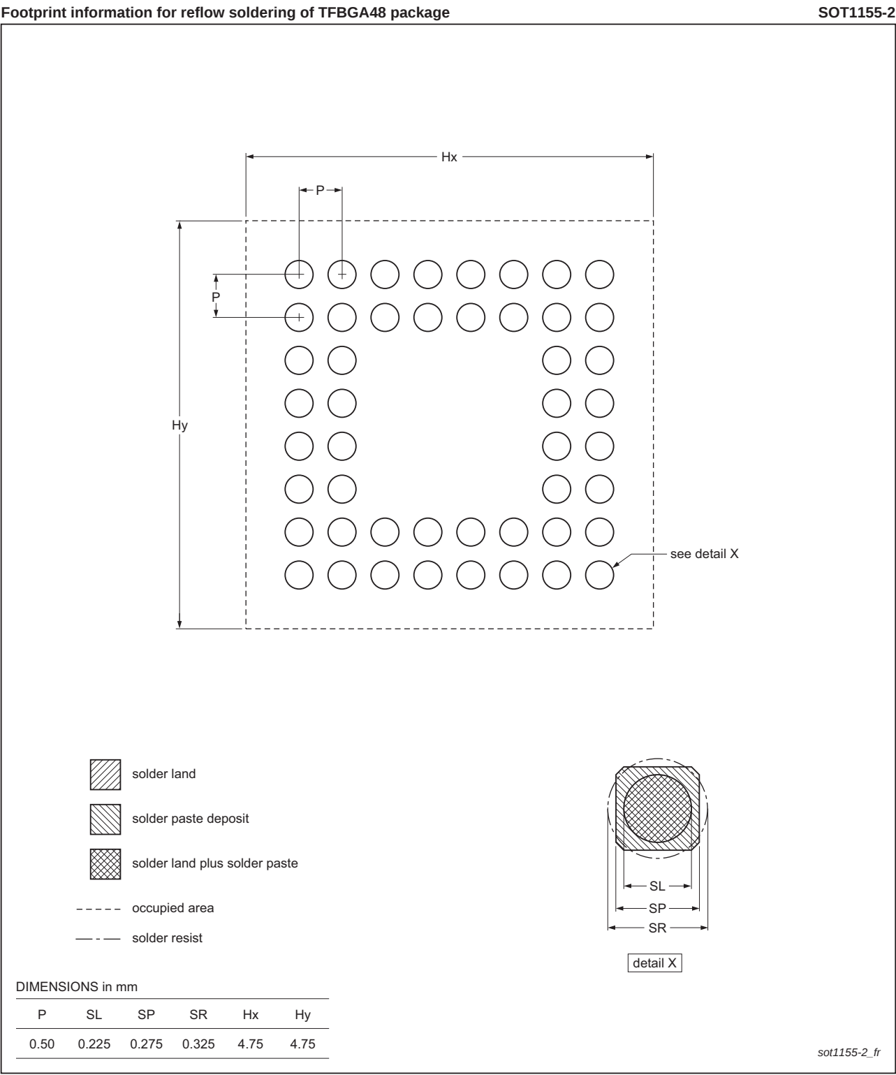
Fig 70. Reflow soldering for the TFBGA48 package
