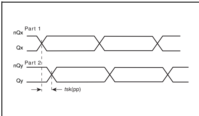
Part-to-Part Skew
