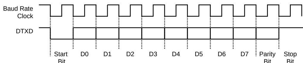
Figure 26-9. Character Transmission
