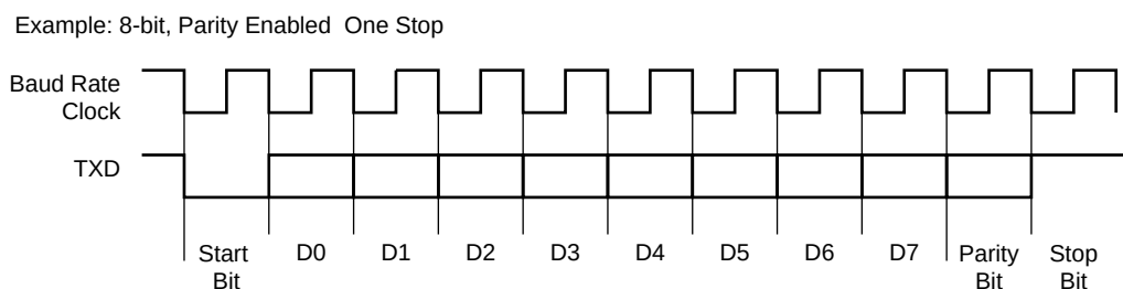
Figure 31-8. Character Transmit
