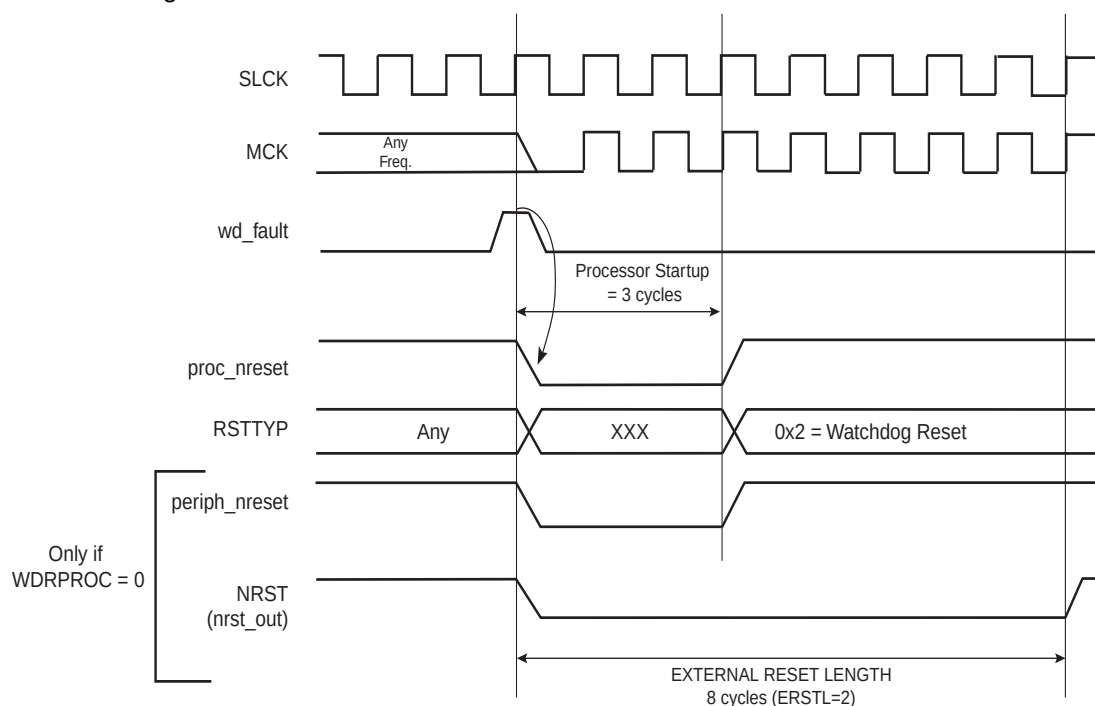
Figure 13-8. Watchdog Reset
