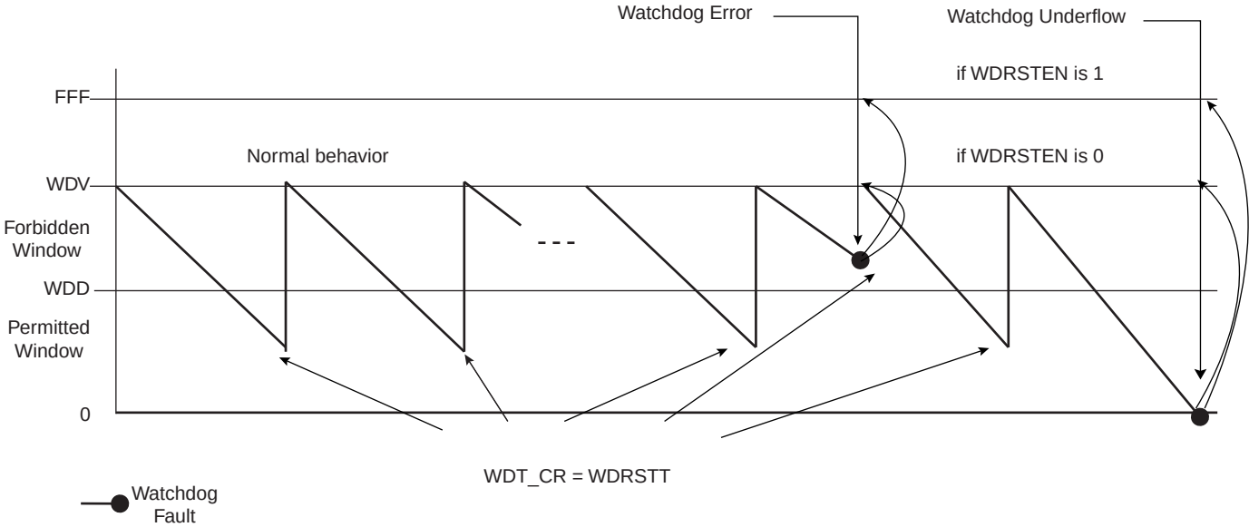
Figure 16-2. Watchdog Behavior
