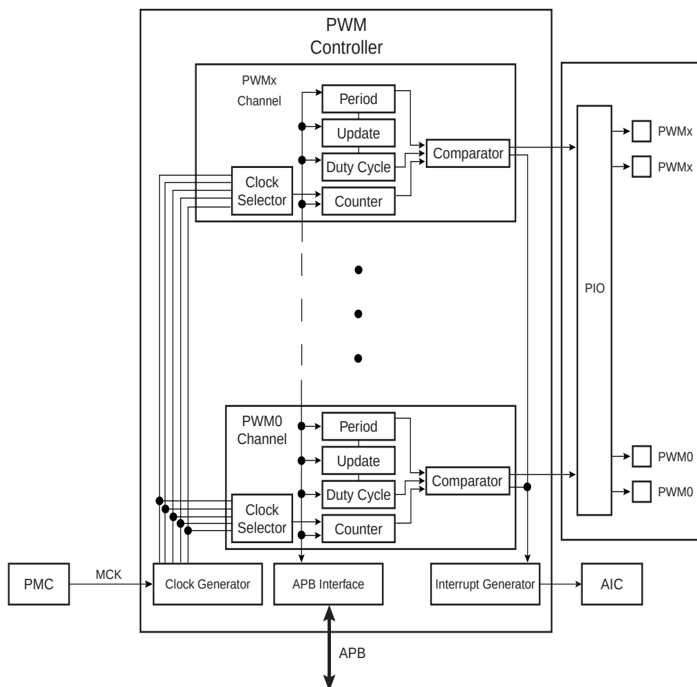
Figure 34-1. Pulse Width Modulation Controller Block Diagram
