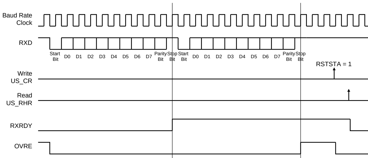
Figure 31-13. Receiver Status
