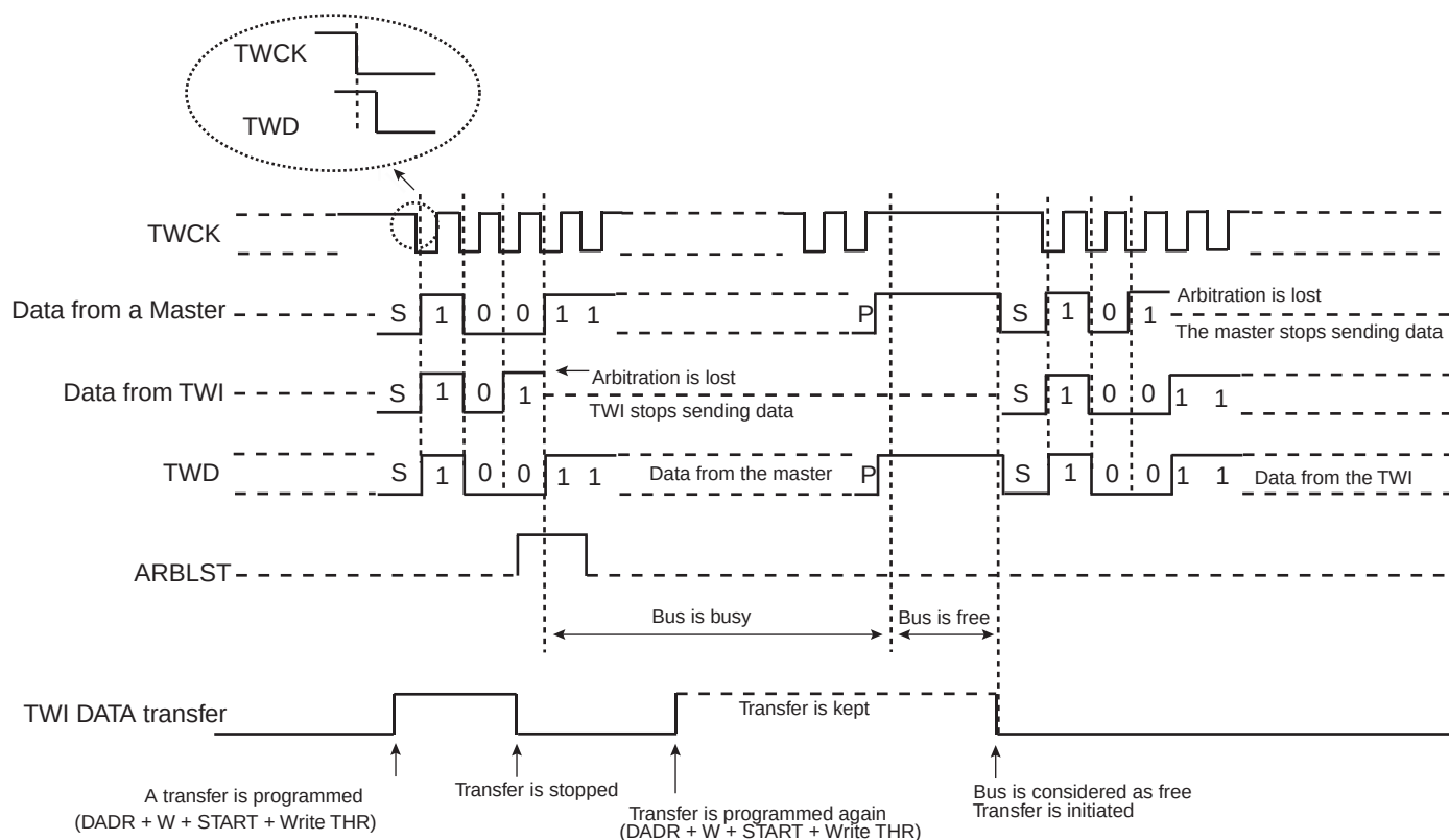
Figure 30-21. Arbitration Cases
