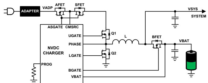
FIGURE 2. NVDC CHARGER CONFIGURATION
