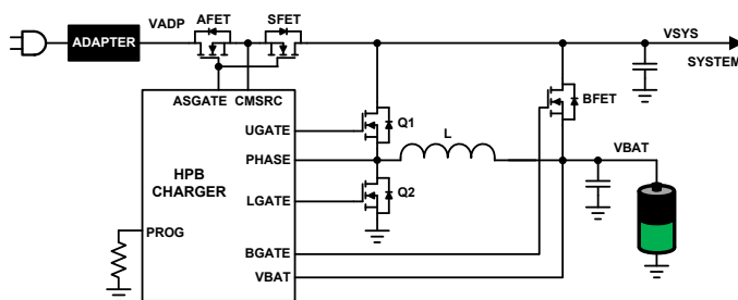
FIGURE 1. HPB CHARGER CONFIGURATION
