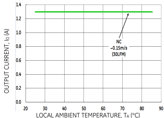
Figure 15. Output Current Derating for the Open Frame SHHD003A0A in the Transverse Orientation; Airflow Direction from Vin(-) to Vin(+); Vin = 48V.
