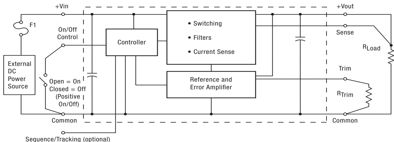
Figure 1. OKX2-T/10, -T/16
