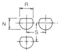
Mounting Details
