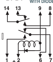
DPDT
