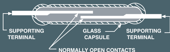
Figure 1. Construction of Switch Capsule of Typical Dry Reed switch (SPST-NO)
