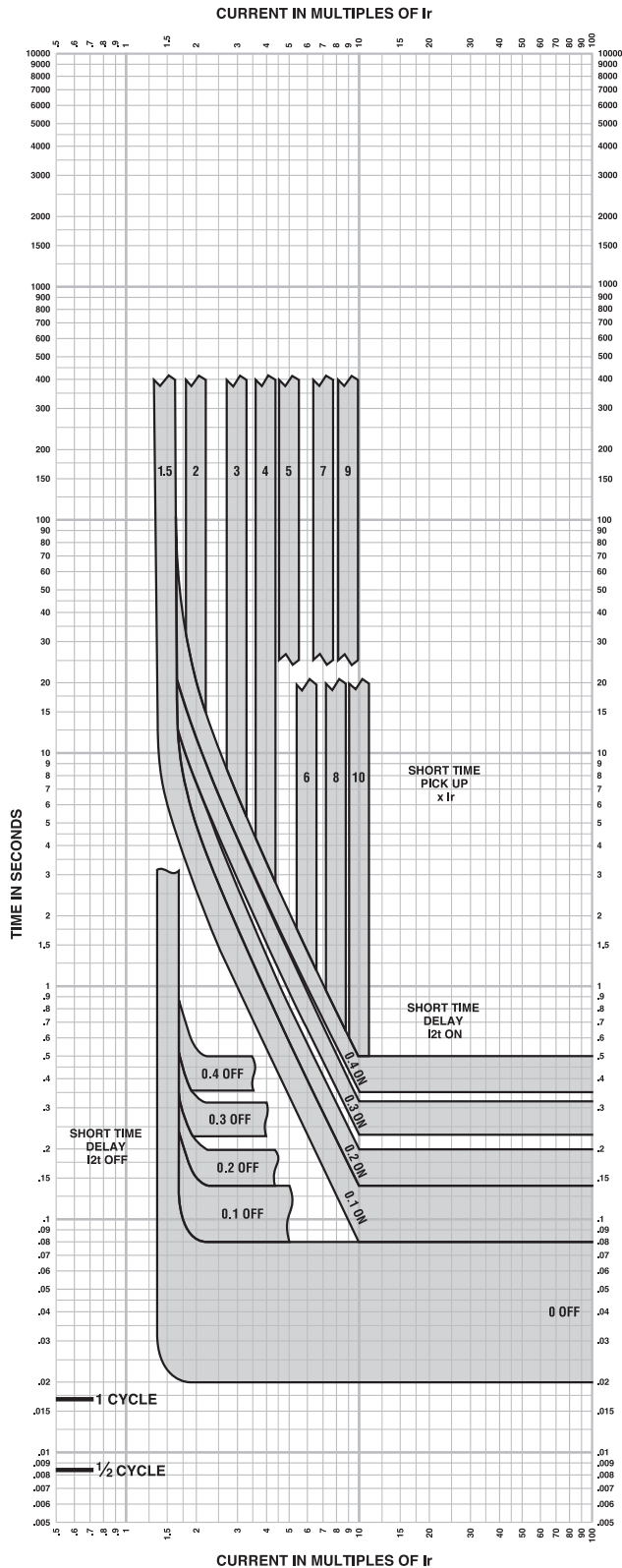
Figure 92: Micrologic 5.2A/5.2E/6.2A/6.2E Electronic Trip Unit Short Time Trip Curve
