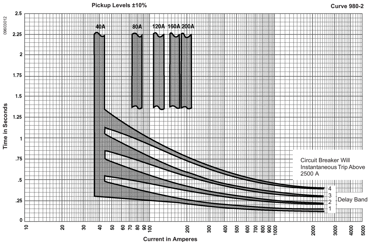
Figure 78: Ground Fault Module GFM250JD Trip Curve
