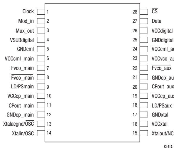
Figure 2. SKY72301-22 Pinout, 28-Pin EP-TSSOP (Top View)
