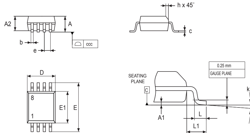
Figure 28. SO8N – Outline
