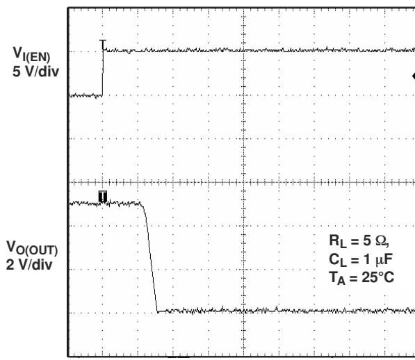
Figure 6-31. Turnoff Delay and Fall Time With 1-μF Load
