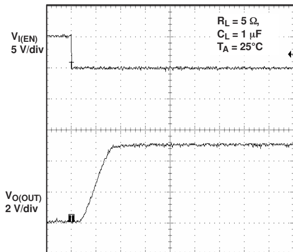
Figure 6-30. Turnon Delay and Rise Time With 1-μF Load
