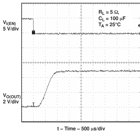
Figure 6-32. Turnon Delay and Rise Time With 100-μF Load
