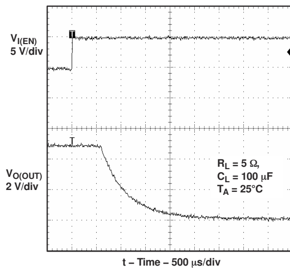
Figure 6-33. Turnoff Delay and Fall Time With 100-μF Load
