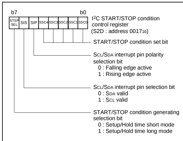
Fig. 45 Structure of I²C START/STOP condition control register
