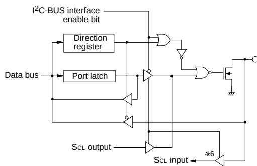
(27) Port P77
