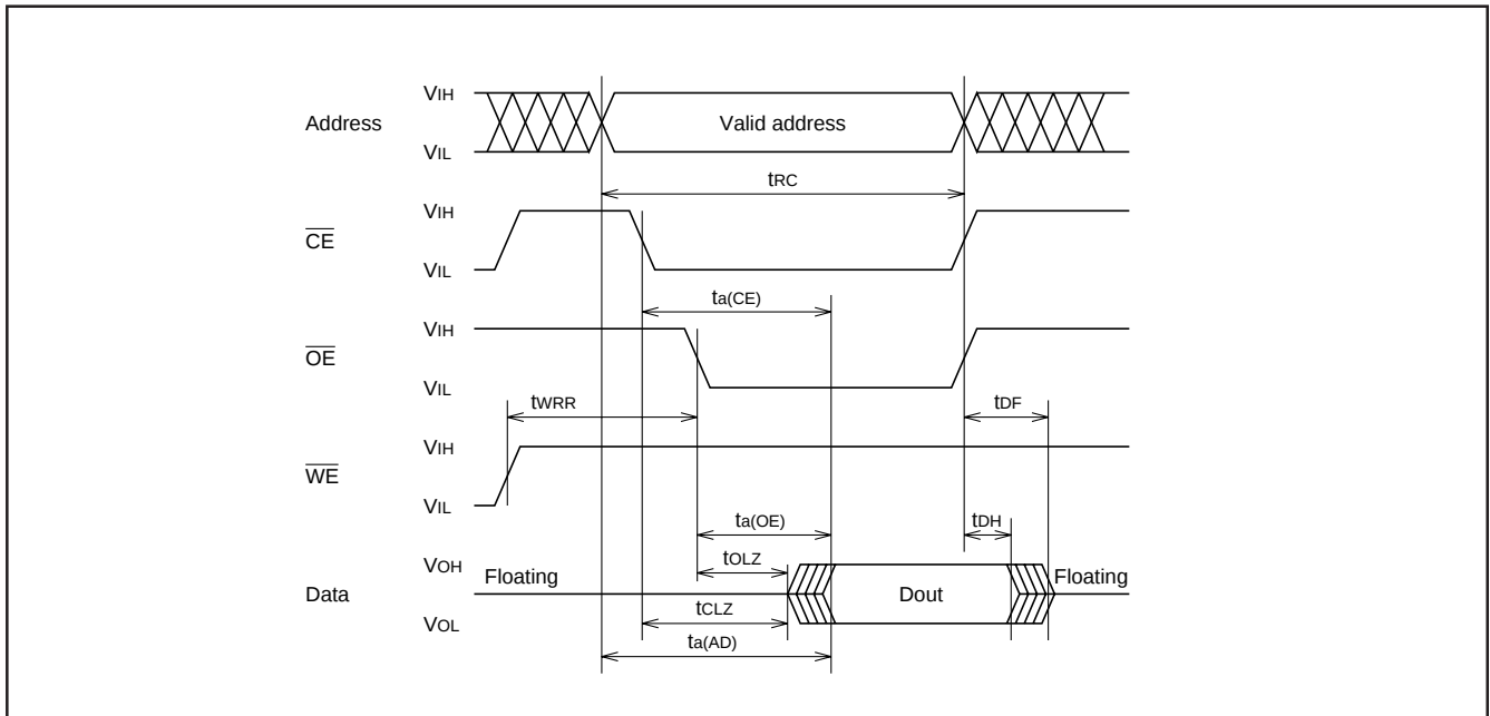
Fig. 67 Read timing
