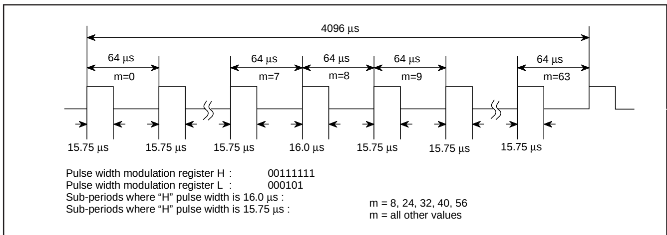
Fig. 30 PWM timing
