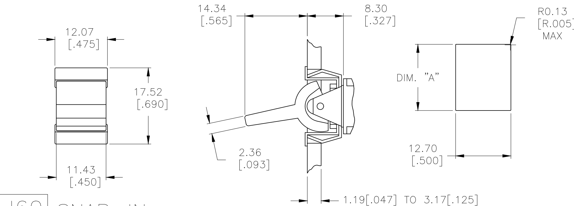
J60 SNAP-IN
