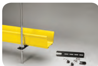
Existing Threaded Rod Bracket Kit (FGS-HETR-XX shown alone and attached to threaded rod)
