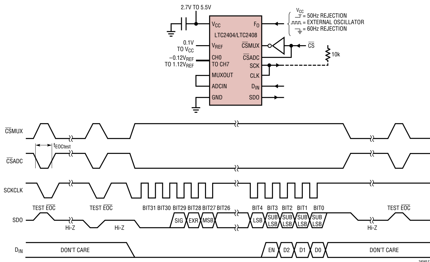
Figure 10. Internal Serial Clock Timing Diagram
