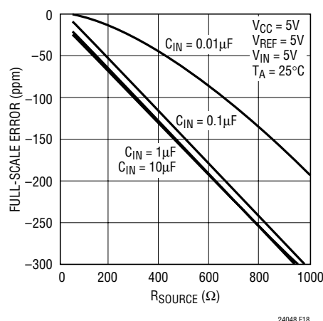
Figure 18. Full-Scale Error vs R_{SOURCE} (Large C)
