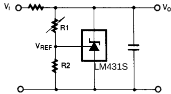
Figure 15. Shunt Regulator
