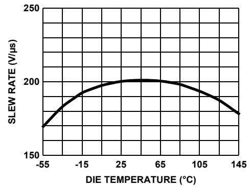
FIGURE 24. SLEW RATE vs DIE TEMPERATURE
