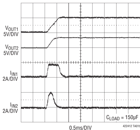
Normal Power-Up Waveform
