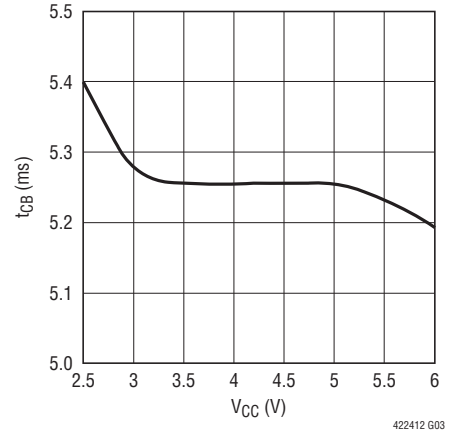
Circuit Breaker Delay vs V_{CC}
