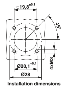
Installation dimensions
