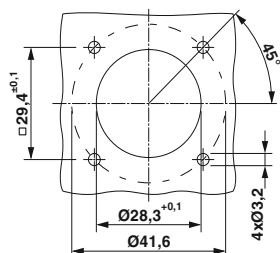
Installation dimensions for short and long design
