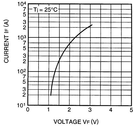
FORWARD CHARACTERISTICS (TYPICAL)
