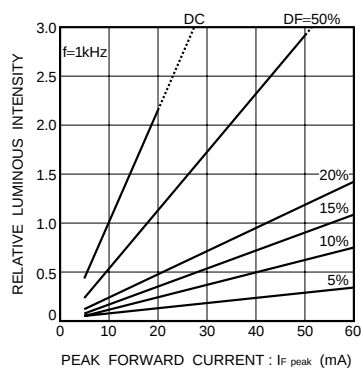
Fig.19 Luminous intensity vs. peak forward current
